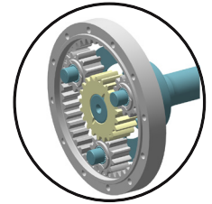
Planetary Drive
